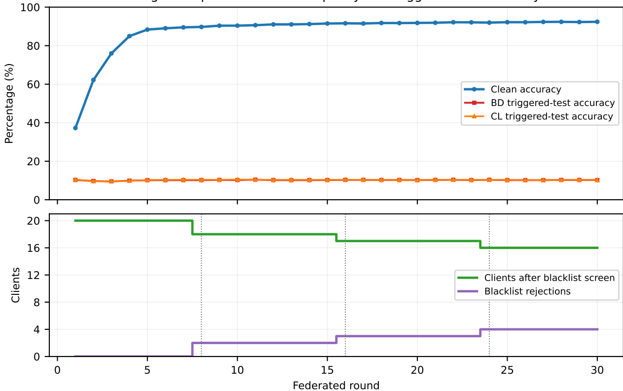
Single completed run: model quality and triggered-test accuracy
